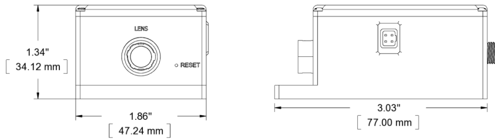
LC-1S Dimensions
