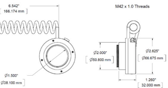
LC-2A-M42 EF-M42x1 Lens Adapter
