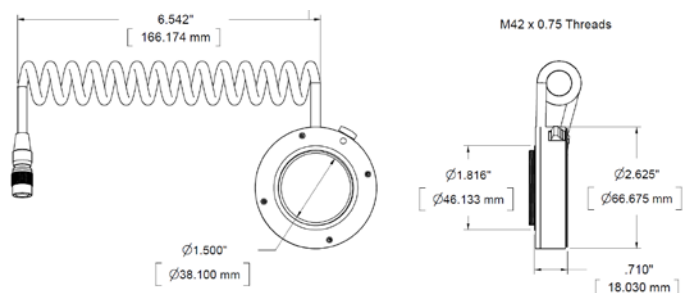
LC-2A-T18 EF-M42x0.75 Lens Adapter
