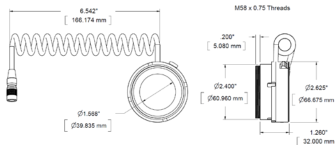
LC-2A-M58-75 EF-M58x0.75 Lens Adapter
