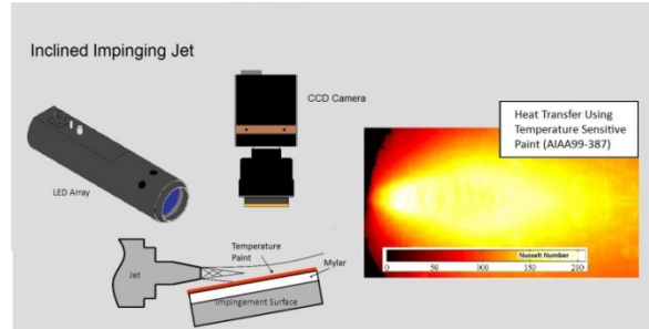
Heat Transfer measurements on the impingement surface of and under-expanded sonic jet impinging at an inclined angle using Temperature Sensitive Paint.
